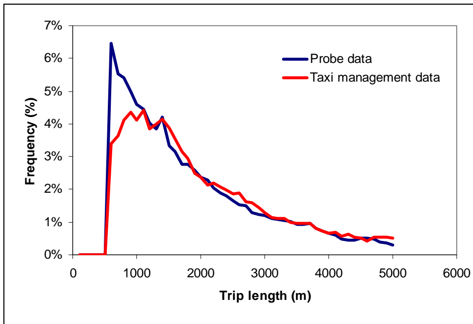
Figure 7 Comparison of trip length distribution
