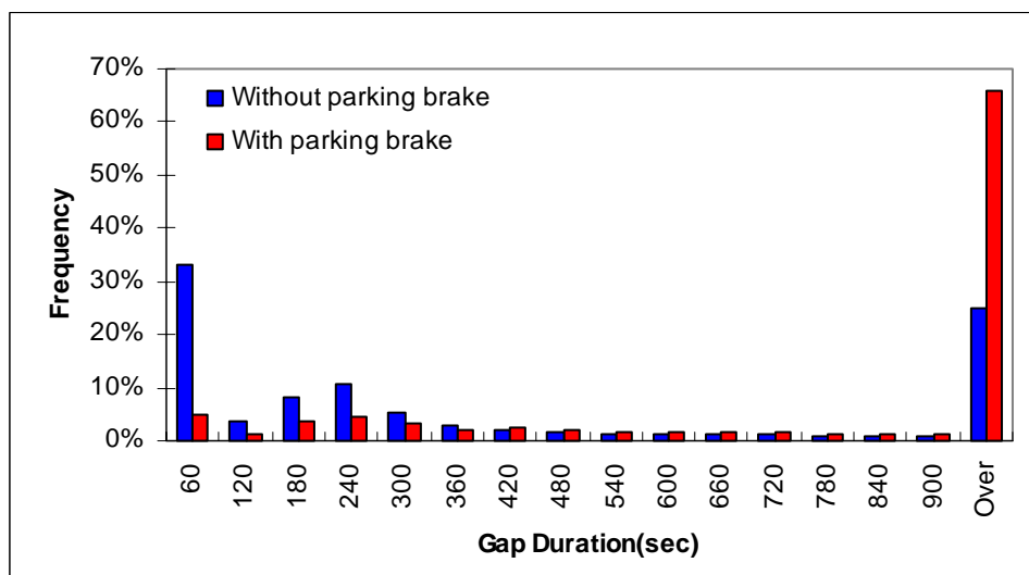
Figure 5 Frequency of gap with parking brakes
